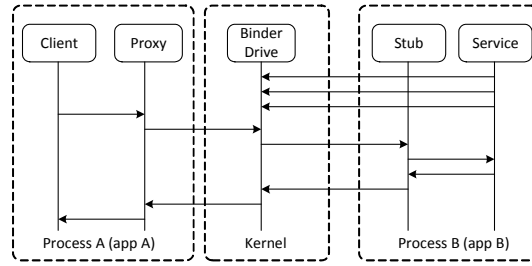
Fig. 4. Workflow of binder using in communication between proxy and service
