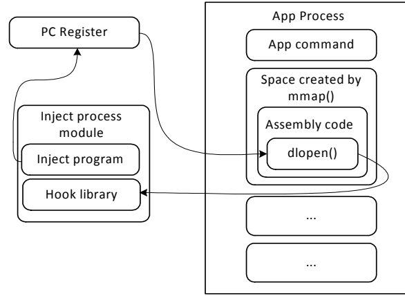
Fig. 2. Injection in an app process
