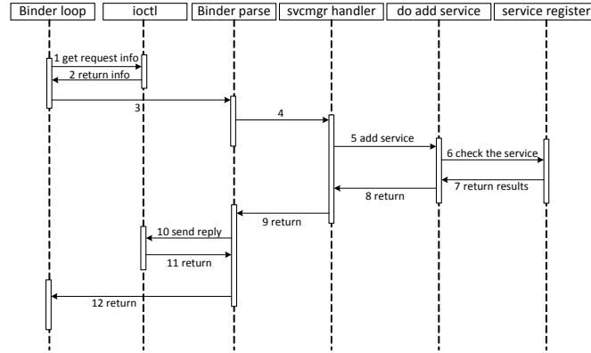
Fig. 3. Find the handle of service in service manager
