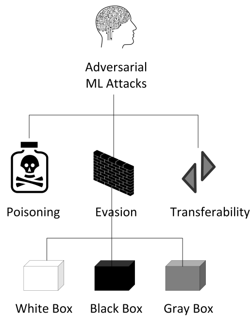
Figure 3. Common Adversarial Machine Learning Attacks
