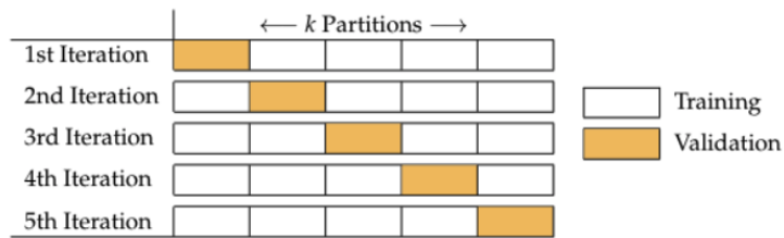
Figure 1. k -fold Cross Validation
